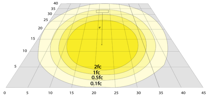
36W, 5000K Area 40'x 45' Mounting Height: 9'
