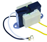
119T86A 24 VAC 20 VA Transformer, with #10 Ring Terminals
