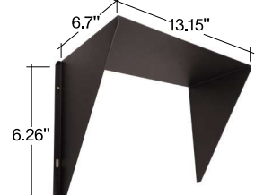
ARL3-240-300W-HSS-BZ
