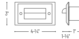
NSW-643/30 Horizontal Shroud
